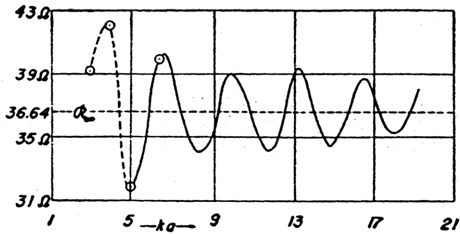
Figure D5- Variation in R_r with disc radius.
