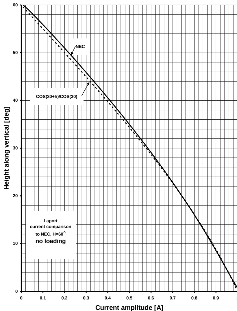
Figure D8 - Comparison of NEC modeling versus Laport for an H=60^\circ unloaded vertical.
