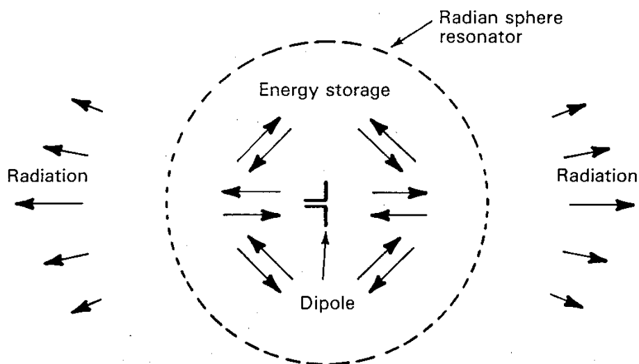
Figure C1 - Radian sphere concept from Kraus [1] .
