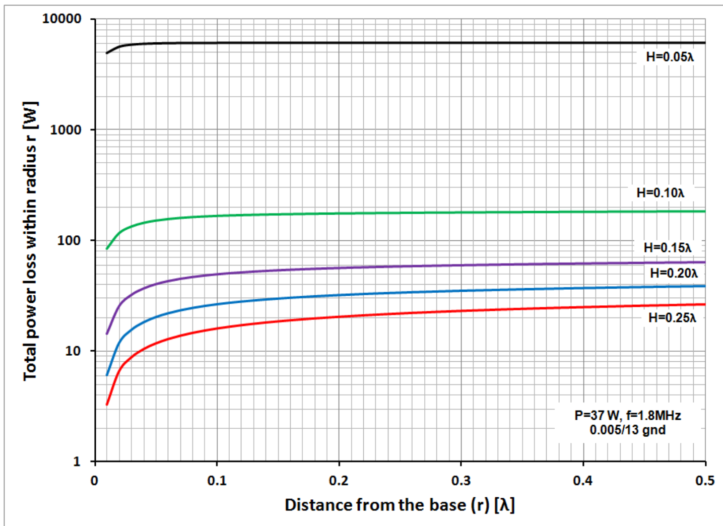
Figure C15 - Total power loss within a given radius r.
