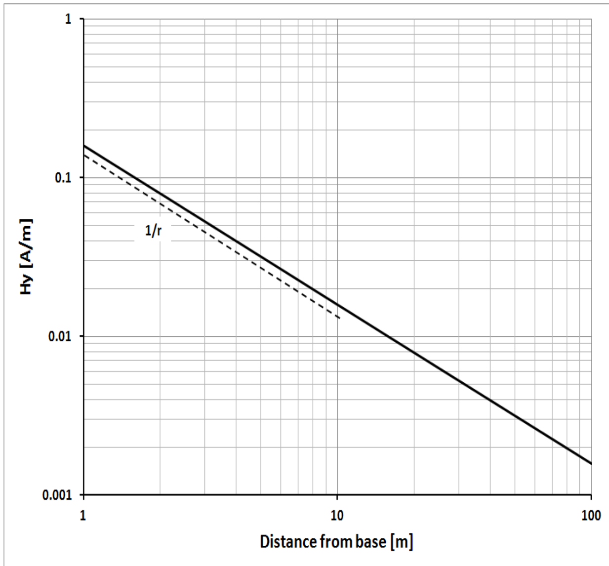
Figure C7- H_\phi as a function of distance radially from a \lambda/4 vertical over perfect ground.
