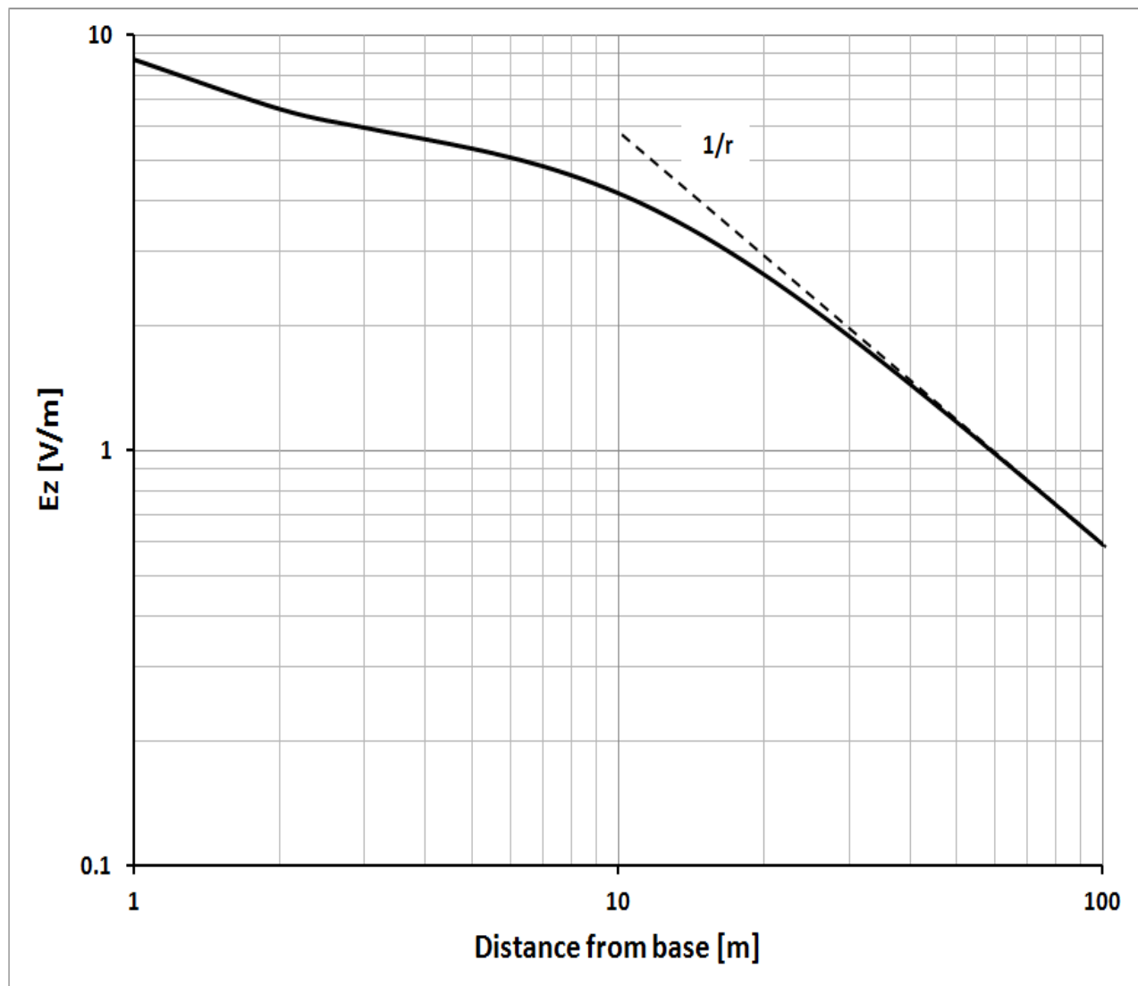
Figure C6 - E_z as a function of distance radially from a \lambda/4 vertical over perfect ground.
