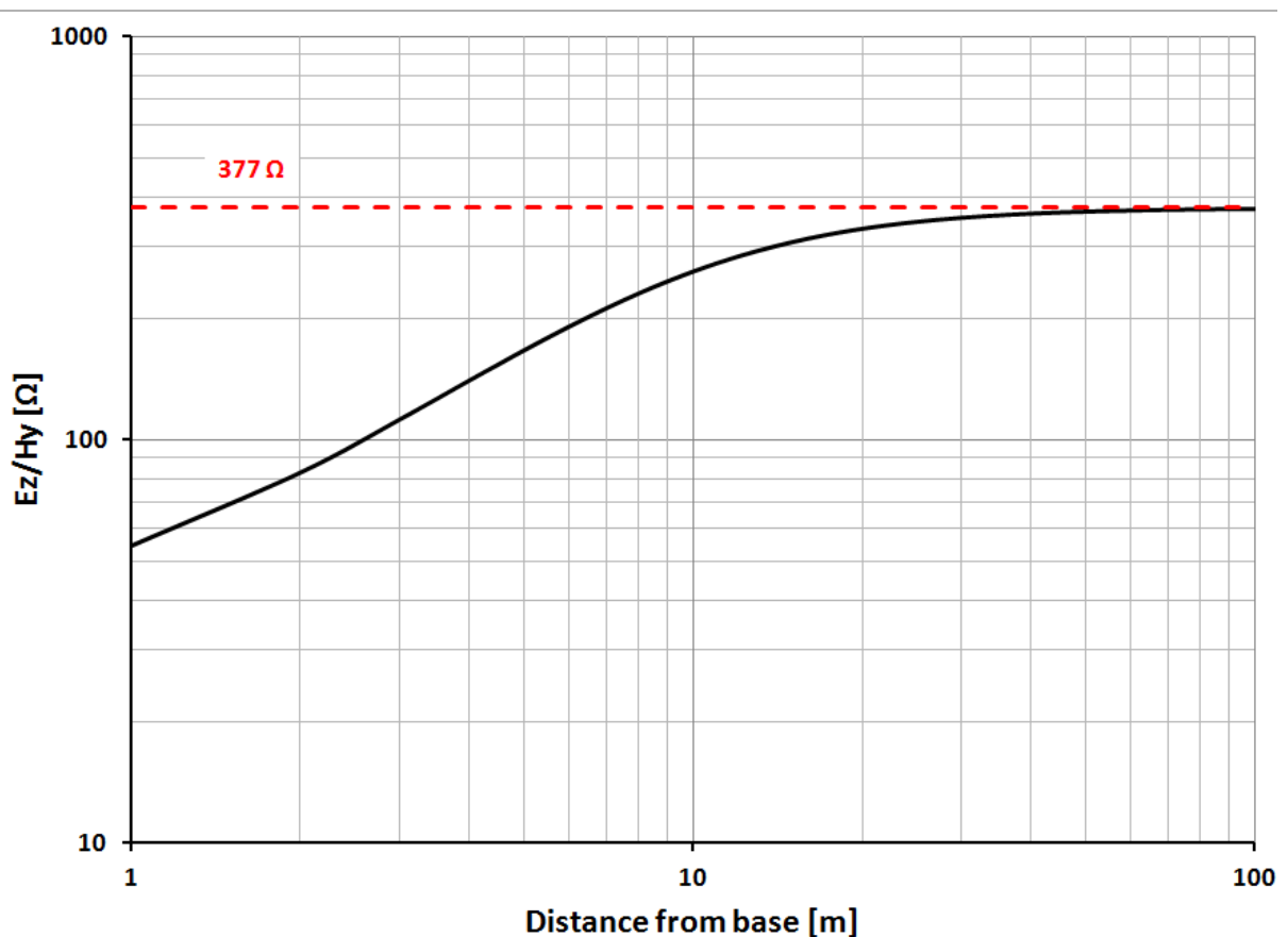
Figure C12 - E_z/H_\phi radially for a \lambda/4 40m vertical over perfect ground.
