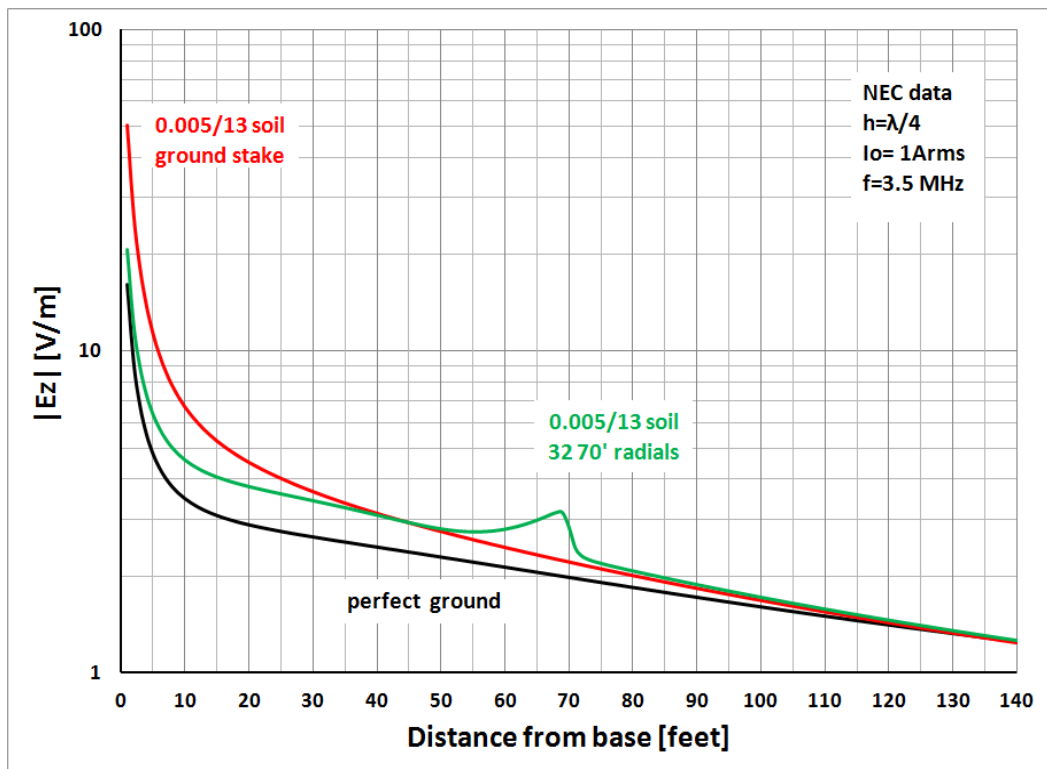
Figure C5 - Comparison of E_z for different ground systems.
