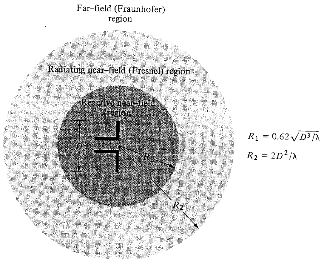
Figure C3 - Field zones (From Balanis [2])
